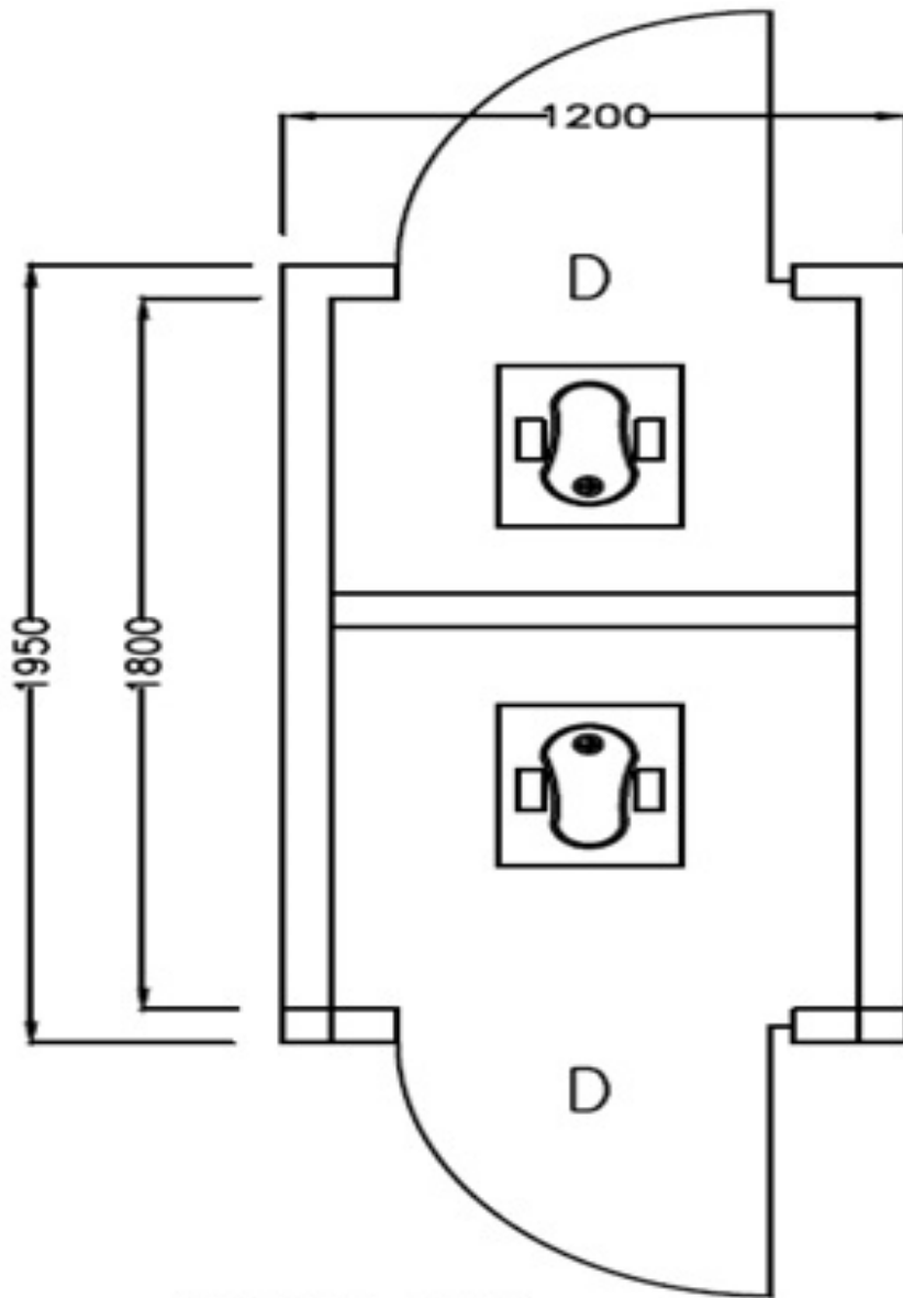
LAYOUT PLAN
